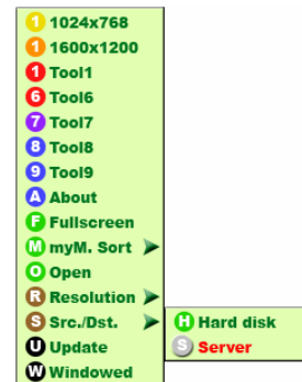
Figure 4: myMenu
