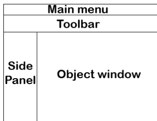
Figure 1: Window layout
