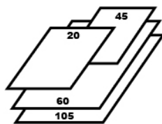
Figure 2: Layer principle
